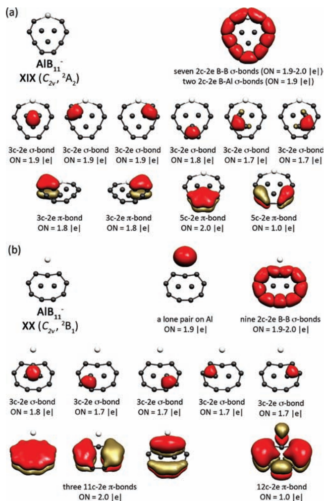
Figure 6. Chemical bonding analysis of the two lowest energy structures of AlB 11 - at the AdNDP/B3LYP/3-21G//B3LYP/6-311+G* level: (a) isomer XIX (C 2v , 2 A 2 ), (b) isomer XX (C 2v , 2 B 1 ).
